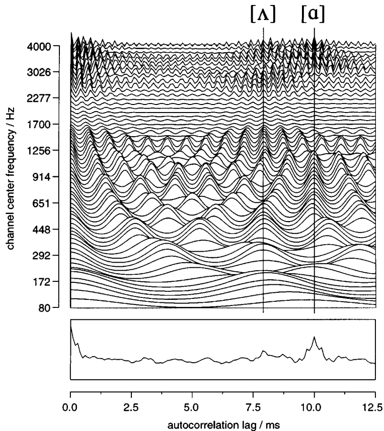
Fig. 3. Autocorrelogram of a synthetic double-vowel pair [ʌ] on a fundamental of 126 Hz and [ɑ] with a fundamental of 100 Hz). The summary correlogram (lower panel) shows a strong peak at an autocorrelation lag of 10 ms, corresponding to periodicities in the signal at harmonics of 100 Hz. A smaller peak at 7.9 ms corresponds to harmonics of 126 Hz.
