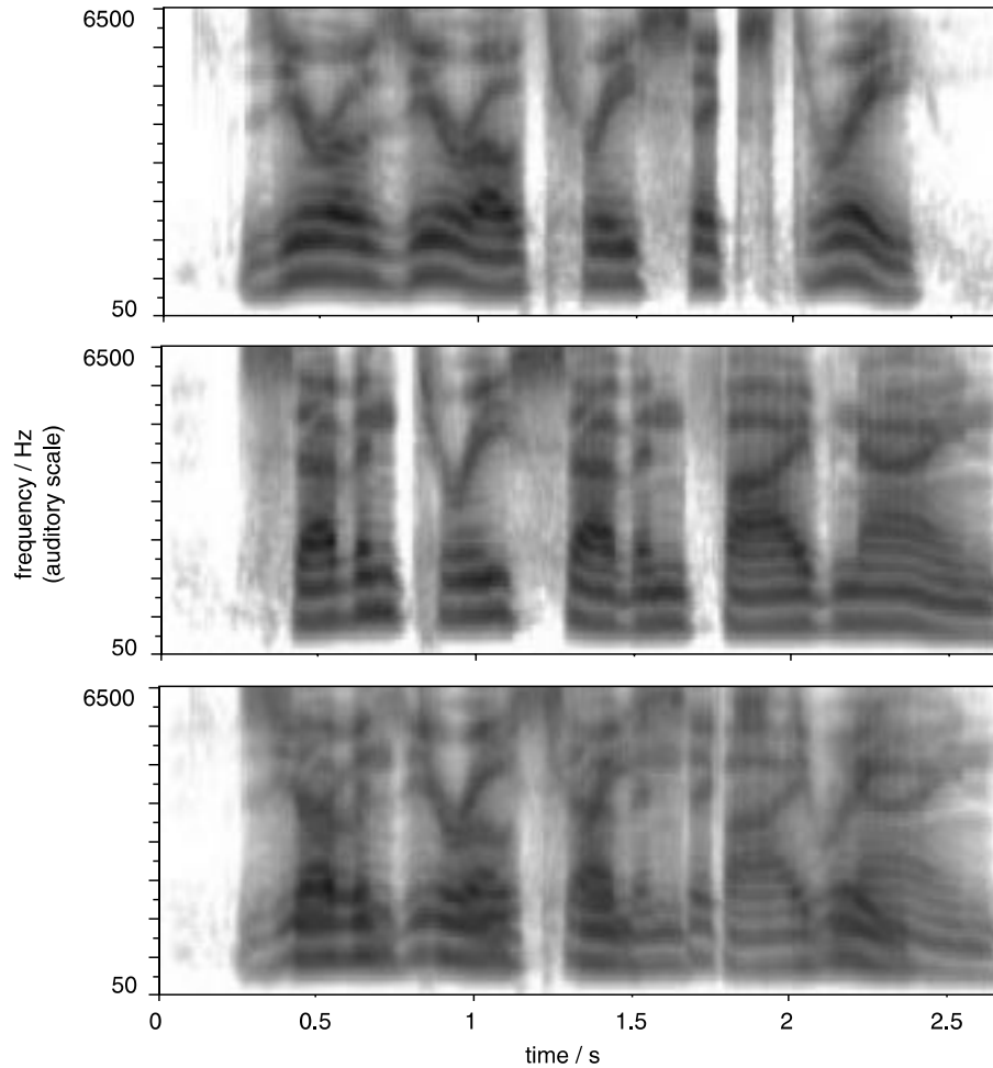
Fig. 1. Auditory spectrograms of spoken digit sequences. Upper: “zero zero three six three”. Middle: “seven three seven five nine”. Lower: mixed signal. Gray-levels are proportional to log-energies at the output of a bank of 64 gammatone filters, equally spaced on an auditory scale (ERB-rate) from 50 to 6500 Hz.
