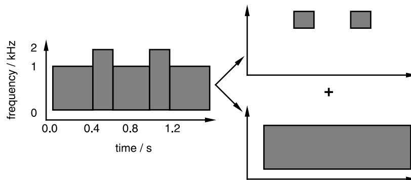
Fig. 5. The old-plus-new principle: schematic representation of the alternating narrow- and broad-band noise stimuli, and its perceptual organization.
